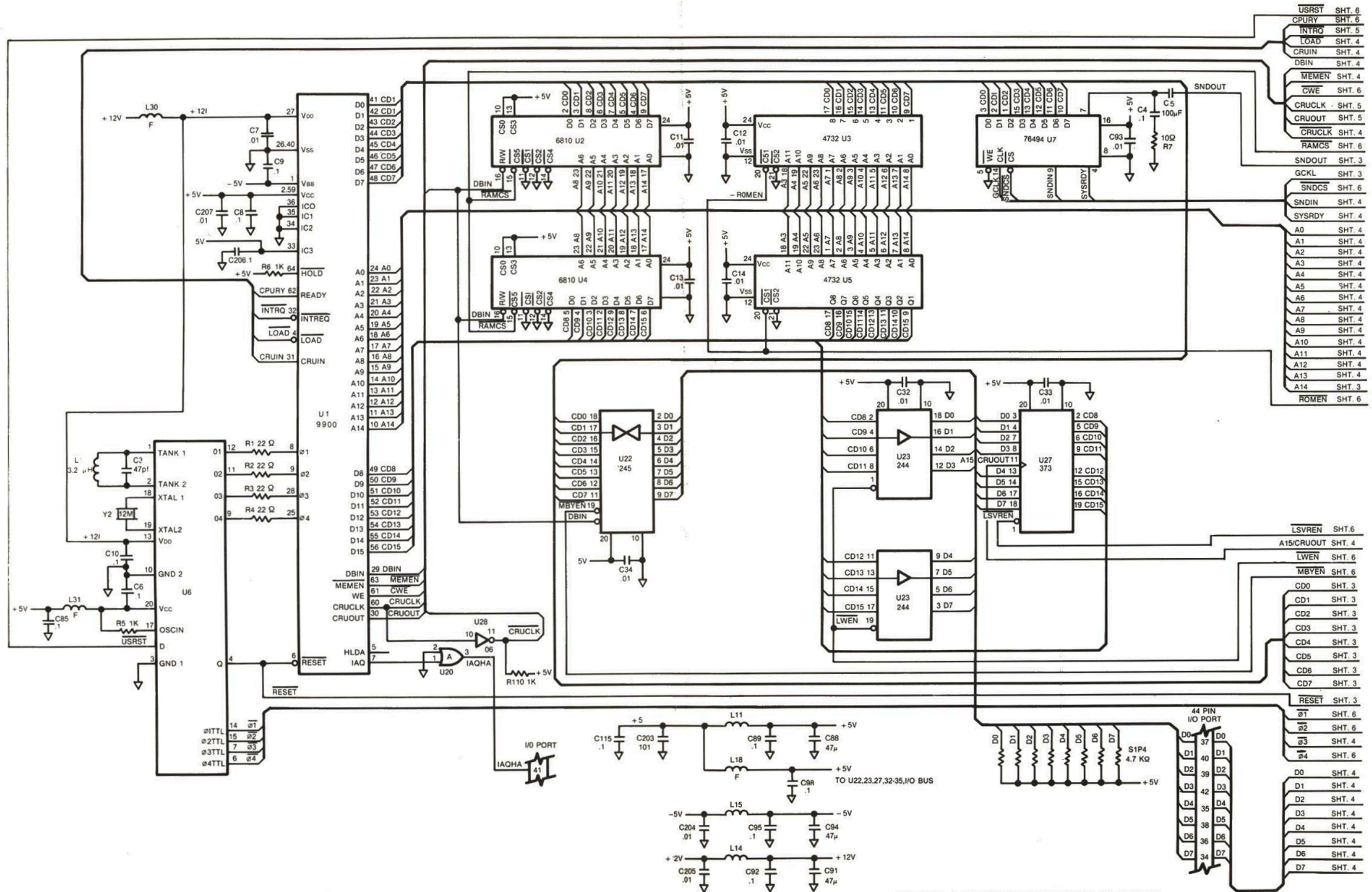
FIGURE J. TI-99/4QI SCHEMATIC DIAGRAM
